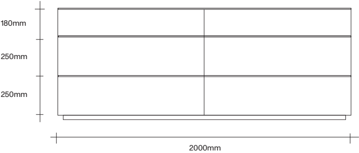
6 Drawer Unit
